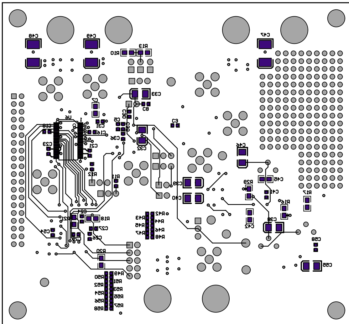
Figure 2–4. Bottom Layer
